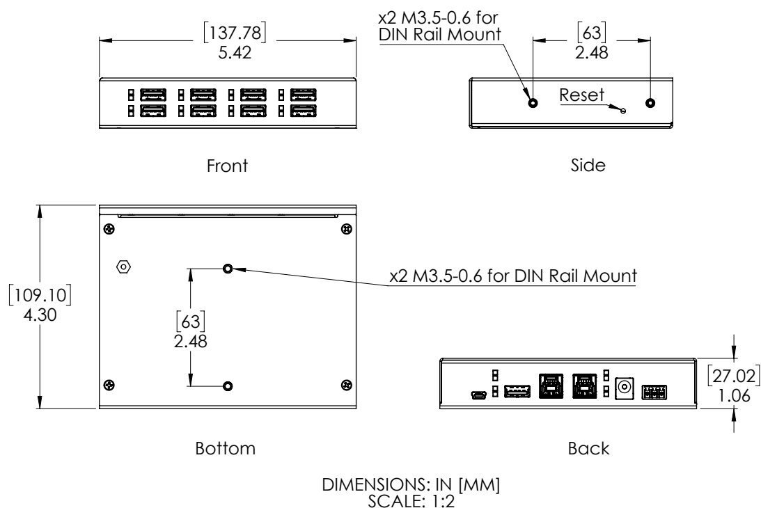
Figure 11: USBHub3+ Mechanical
