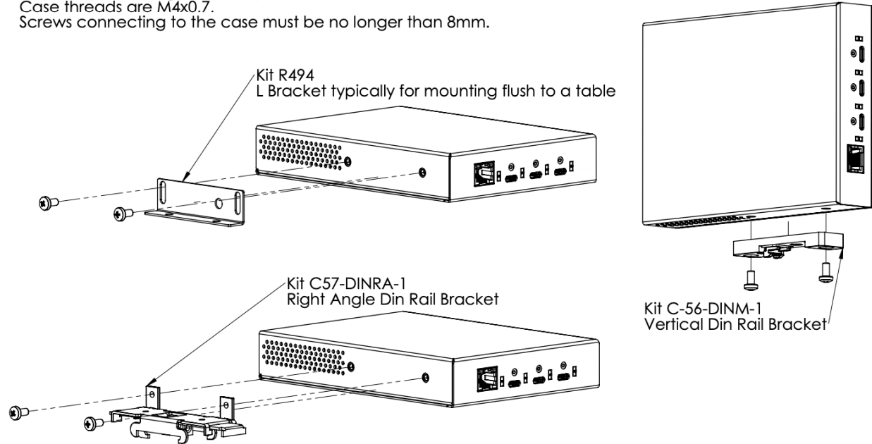
Figure 13: USBExt3c DIN Rail Mount
