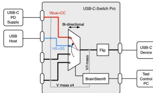
Figure 8: Adding USB-C PD charging capability to a legacy USB host output
