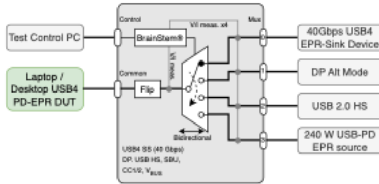
Figure 2: Typical testing application for validation against multiple types of devices
