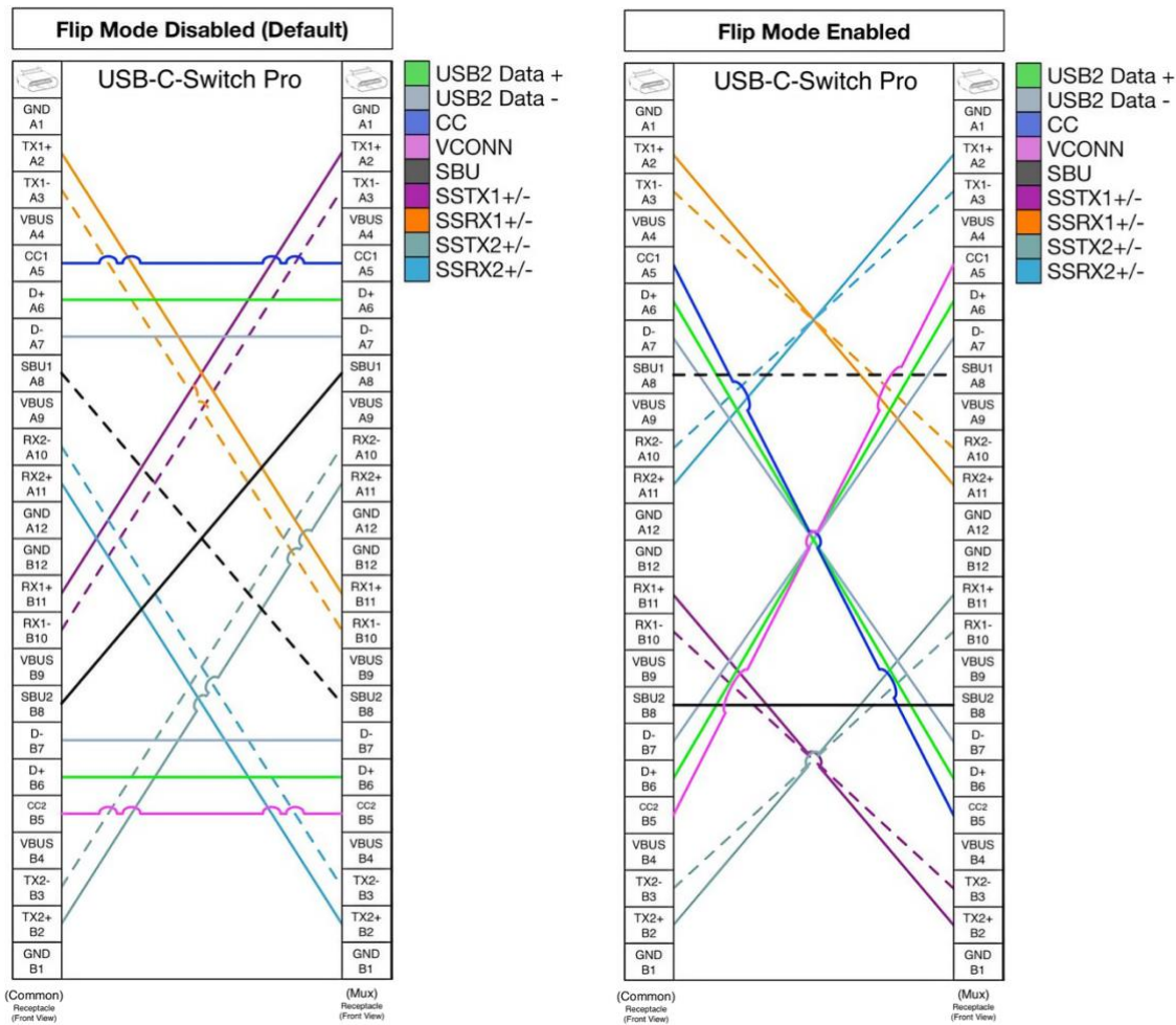
Figure 13: Common-to-Mux port pin mappings
