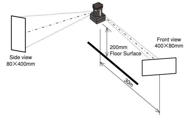
(Figure 1: Spread of laser beam)
