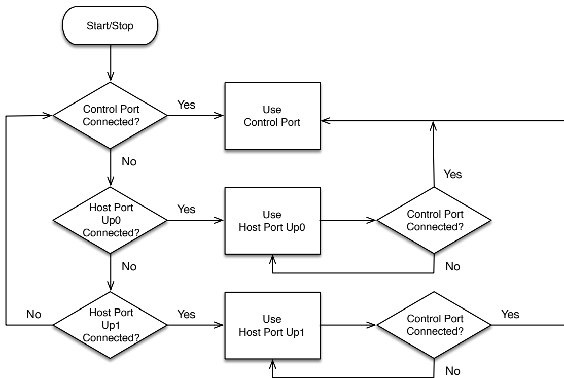
Figure 2: Host Port Control Flow
