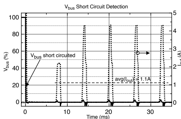
Figure 4: V_{bus} short-circuit mode behavior.
