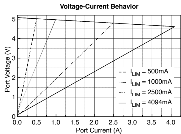
Figure 6: V_{bus} Current Limiting Behavior (V-I)
