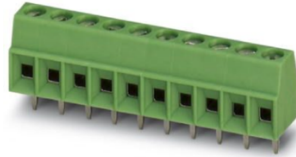
Figure 6: Phoenix Contact 1751329 3.5mm Example Header
