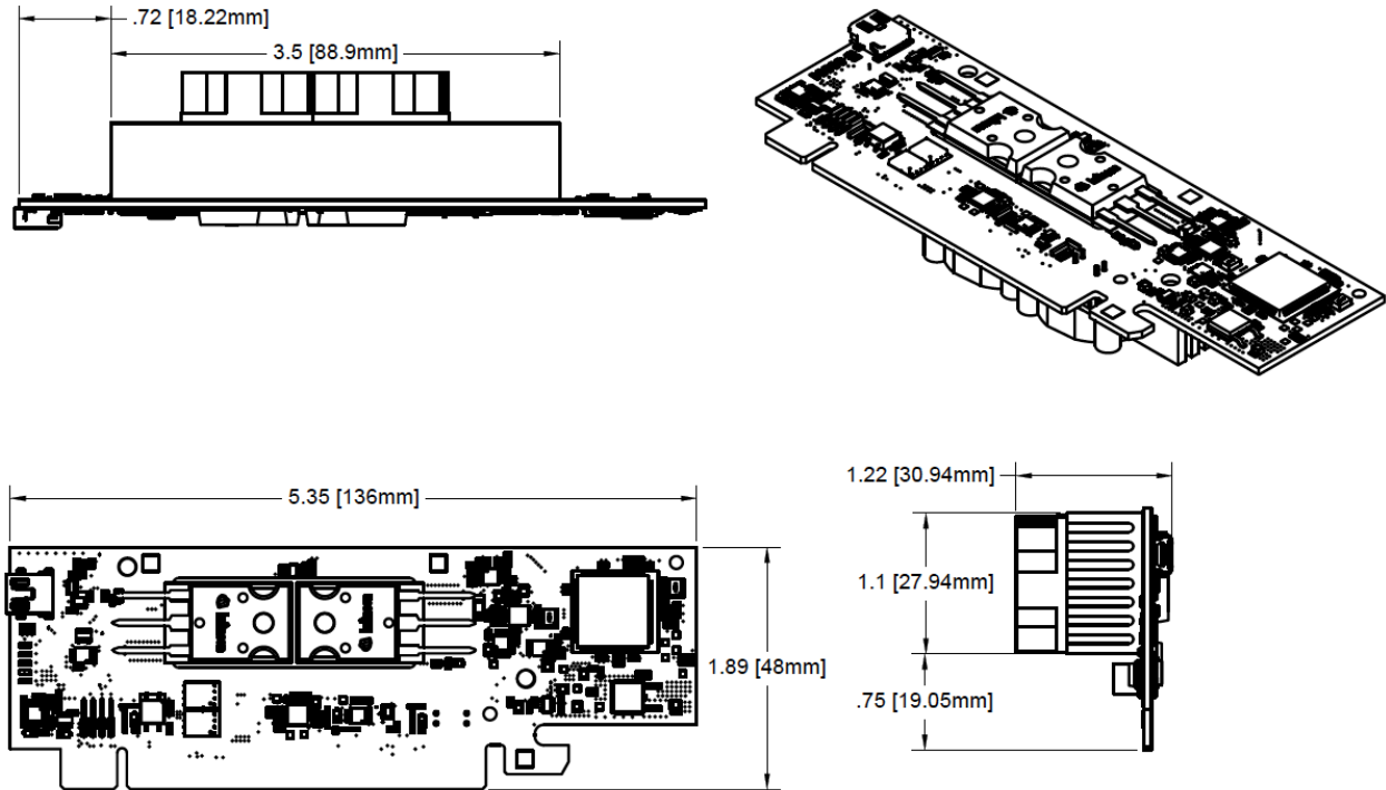
Figure 5: MTM-Load-1 Mechanical
